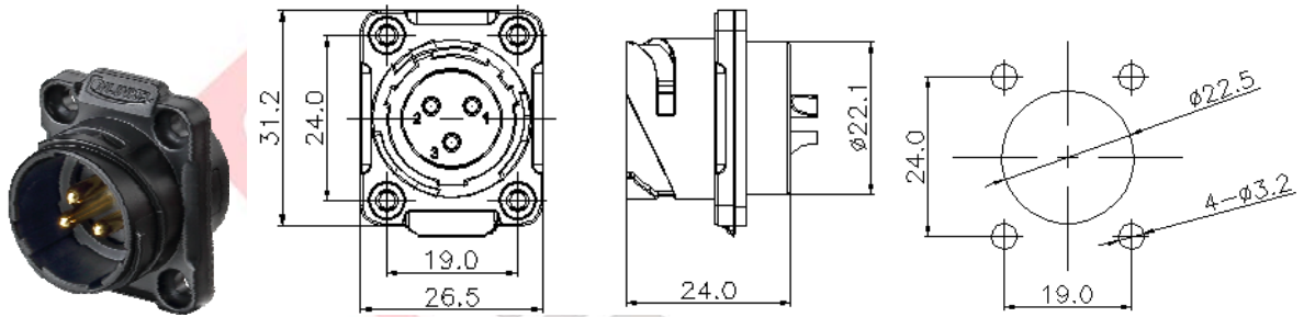
Mounting hole
