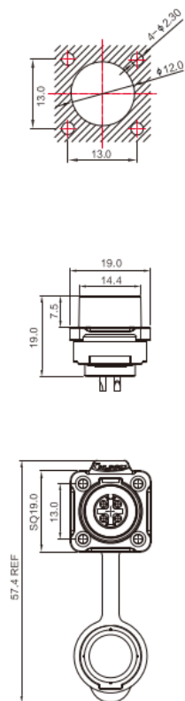
■ Flange Mounting
