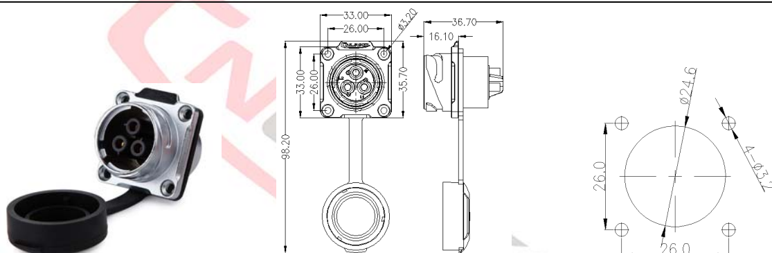
DH-24-J XX _SX-XX-001 Socket
