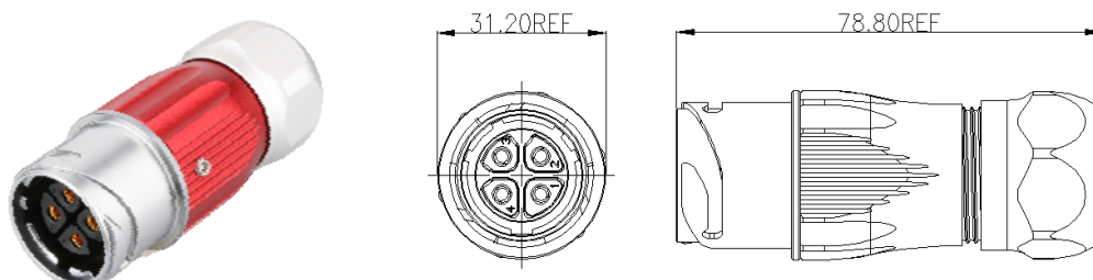
DH-24-J XX PP-XX-001 Butt Socket
