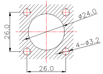
Mounting hole
