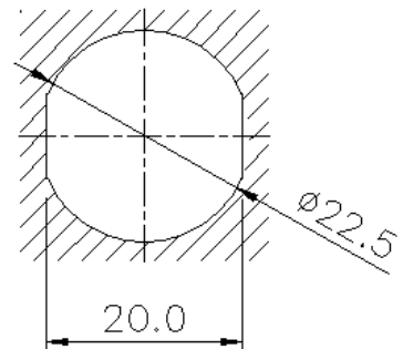
Mounting hole
