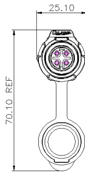
LP-16-J___SX-XX-001 Single hole female socket
