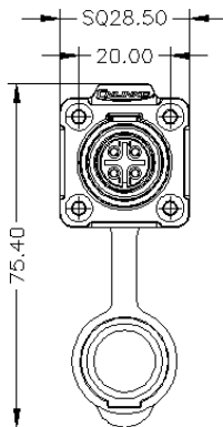
LP-16-J___SX-XX-001 Four holes socket
