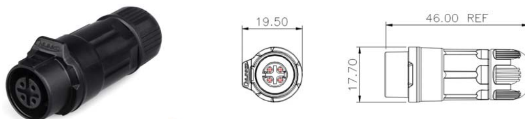
LP-12-J___PP-XX-001 Butt plug
