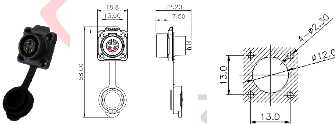
LP-12-J___SX-XX-001 Four holes socket
