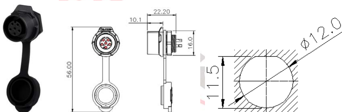
LP-12-J___SX-XX-001 Single hole female socket
