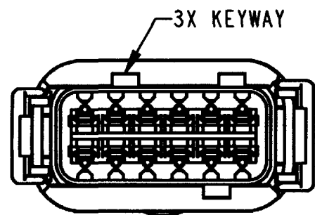
DTM04-12PA KEY -A- COLOR: GREY
