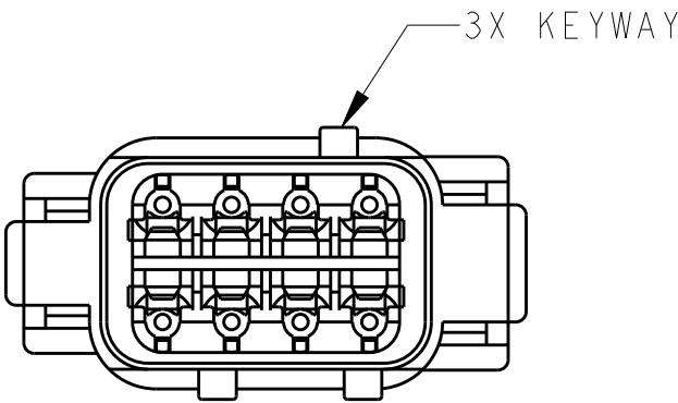
DTM06-08SA KEY -A- COLOR: GREY
