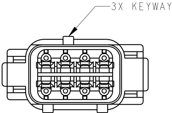
DTM06-08SD KEY -D- COLOR: BROWN
