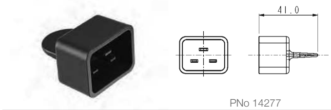
Blanking Cover
