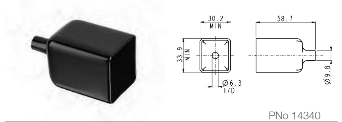
Insulation Boot
