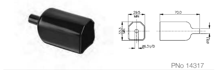
Insulation Boot
