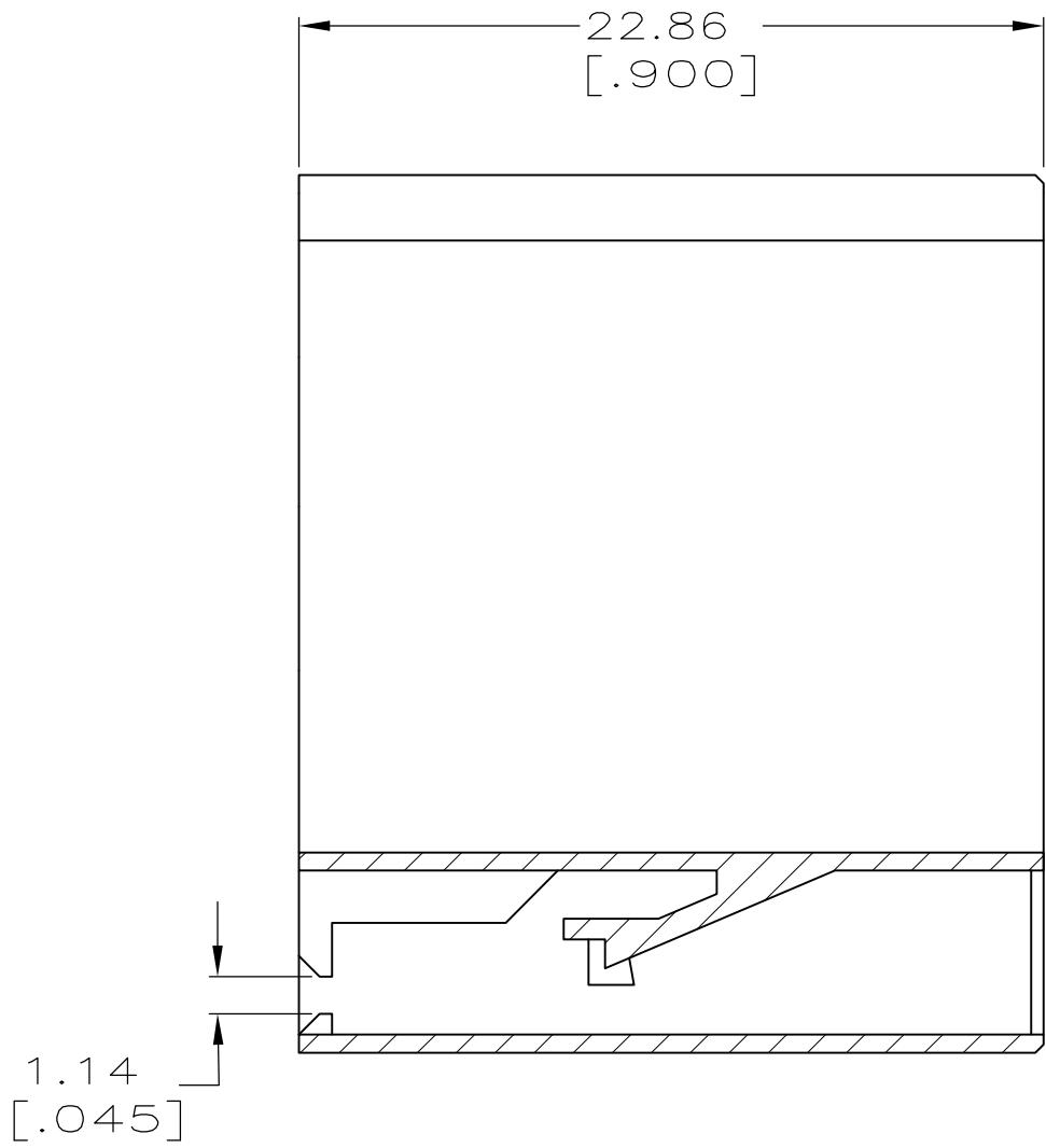
SECTION A—A
