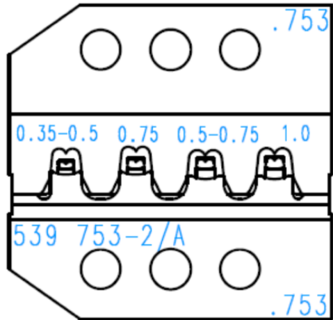
TE Connectivity 539753-2
