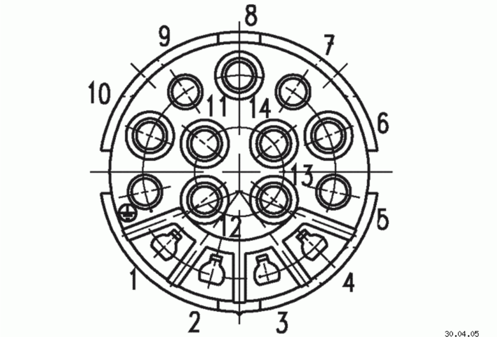
Contact arrangement
