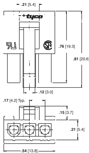
Receptacle Housing
